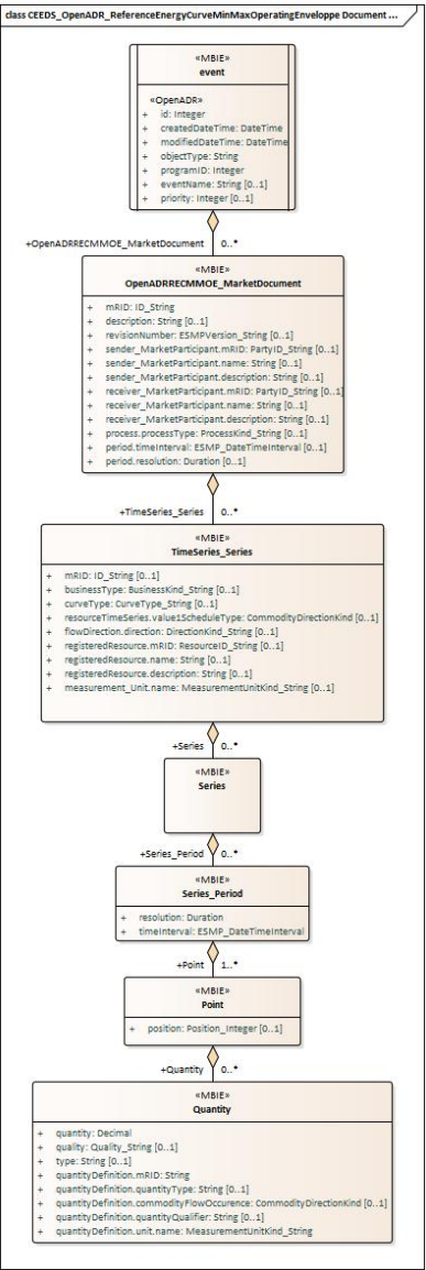
Figure !# - CEEDS_OpenADR_ReferenceEnergyCurveMinMaxOperatingEnvelope Document assembly model
